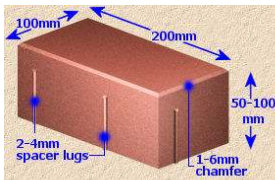
Typical concrete paving block (Product Ref ECP PBT)
